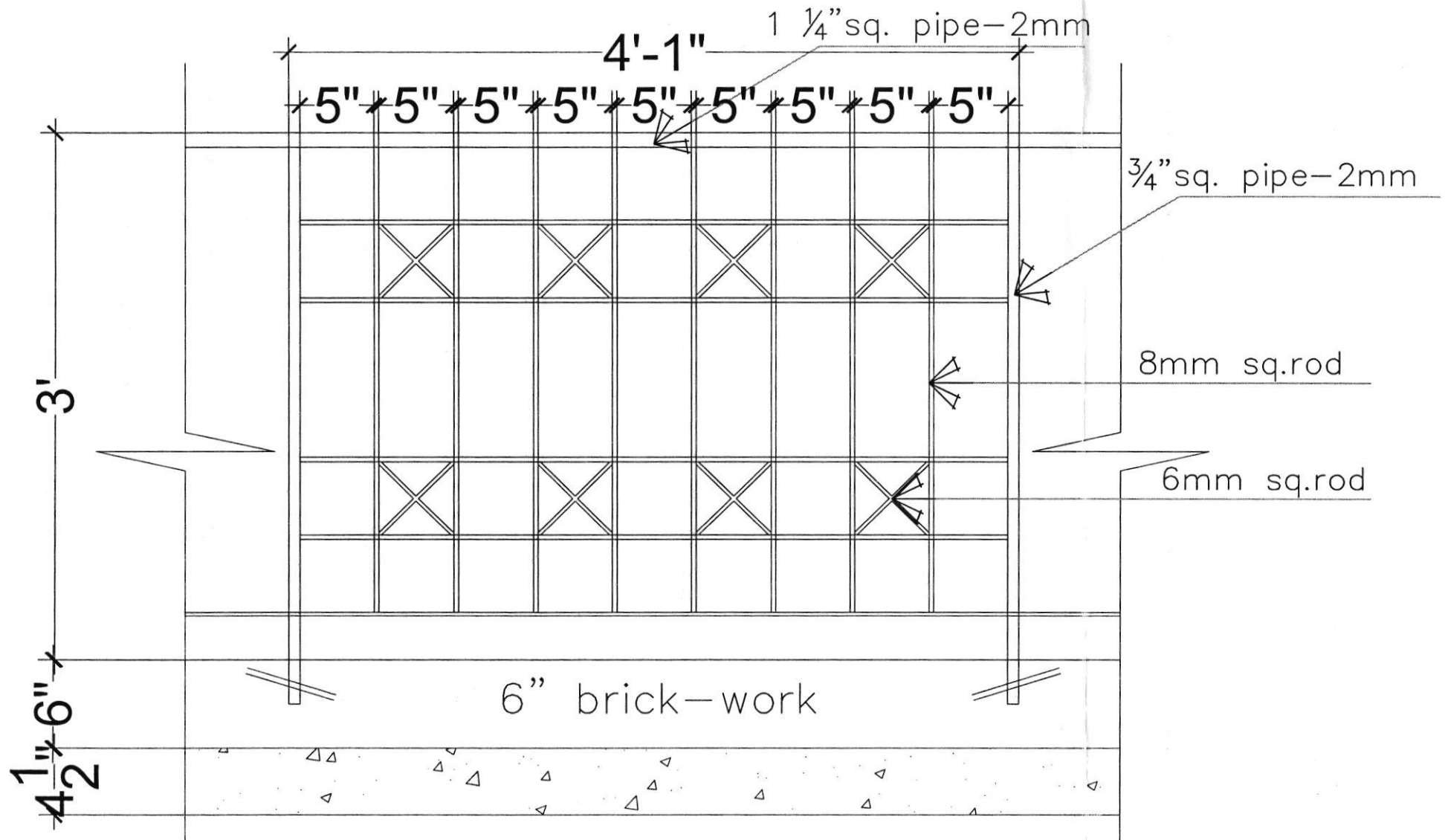
RAILING MODEL 1
