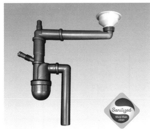
Plumbing Kit-1 Bowl Siphon, Sanitized, fully assembled
