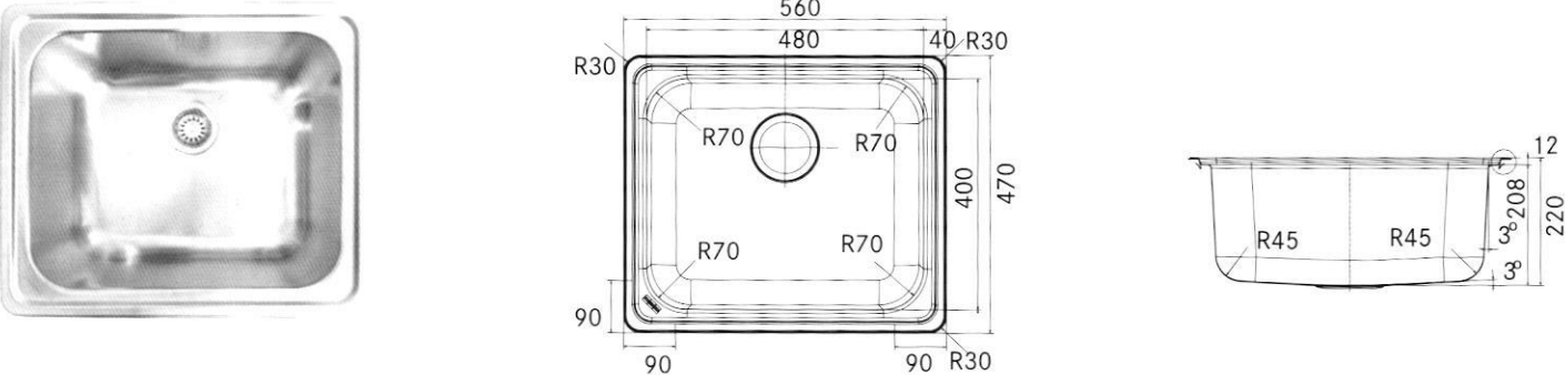
RSX 6 10-56 (22"x18")
