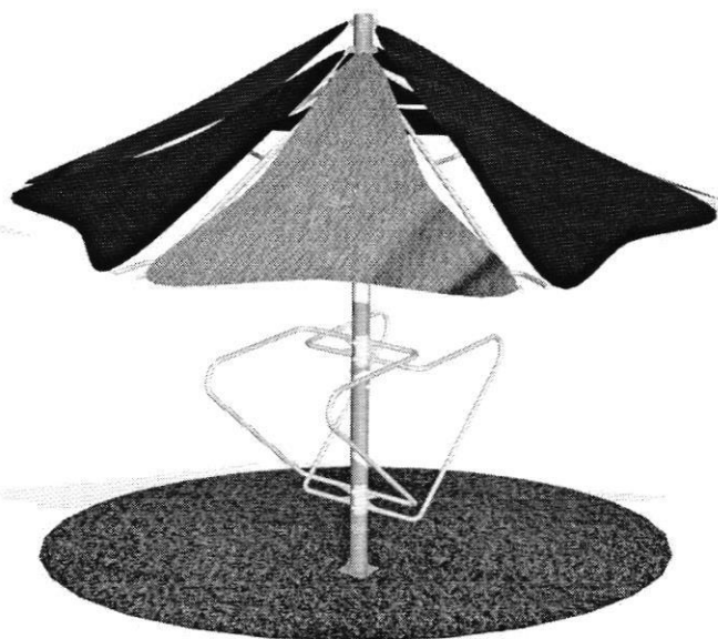
Push-up & Dip Station With Canopy RE-024-GYM Dimension - 4.32 x 4.32 x 3.3 m. (14 x 14 x 10.8 ft.)
