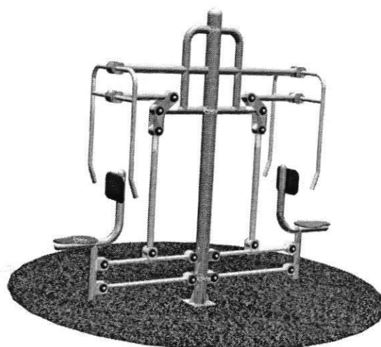
Chest Press Double RE-043-GYM Dimension - 2.45 x 0.75 x 2.25 m. (8 x 2.4 x 7.3 ft.)
