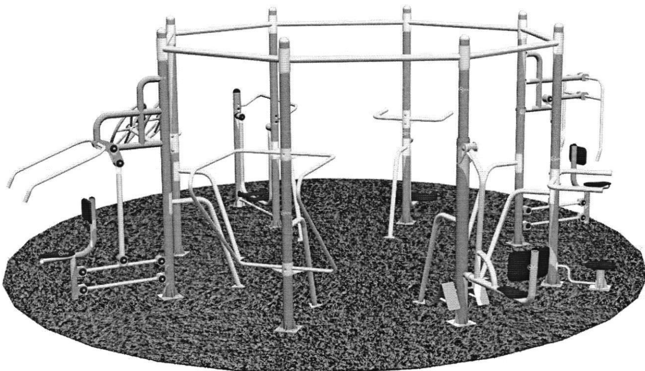
8 Set Fitness Station RE-063-GYM Dimension - 5.5 x 5.5 x 2.57 m. (18 x 18 x 8.4 ft.)
