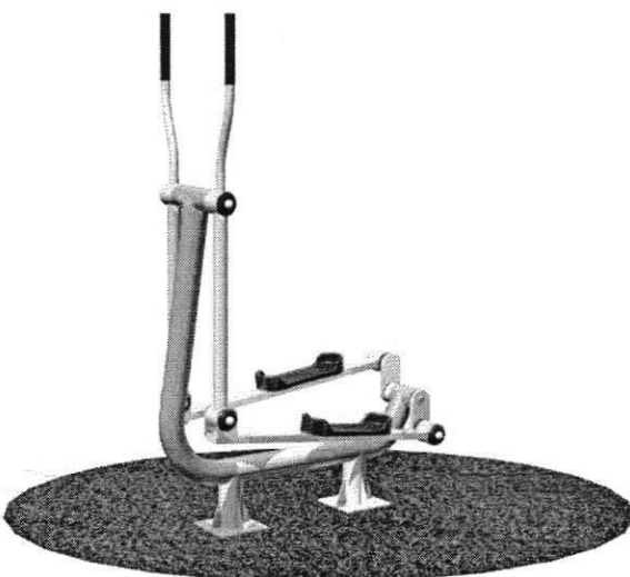
Elliptical Cross Trainer RE-019-GYM Dimension - 1.3 x 0.5 x 1.82 m. (4.2 x 1.6 x 5.9 ft.)
