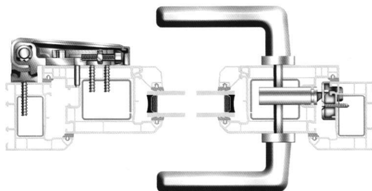
Casement Window with Butt Hinges
