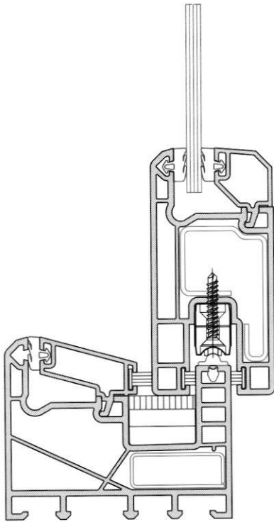
FIXED WITH SINGLE TRACK - "Fix en Slide" (77 mm)
