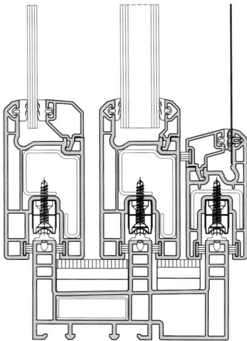
2½ TRACK (102 mm)
