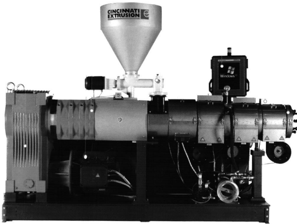
Twin Head Extruder
