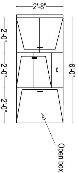
Cabinet-1 ( Depth 24" )
