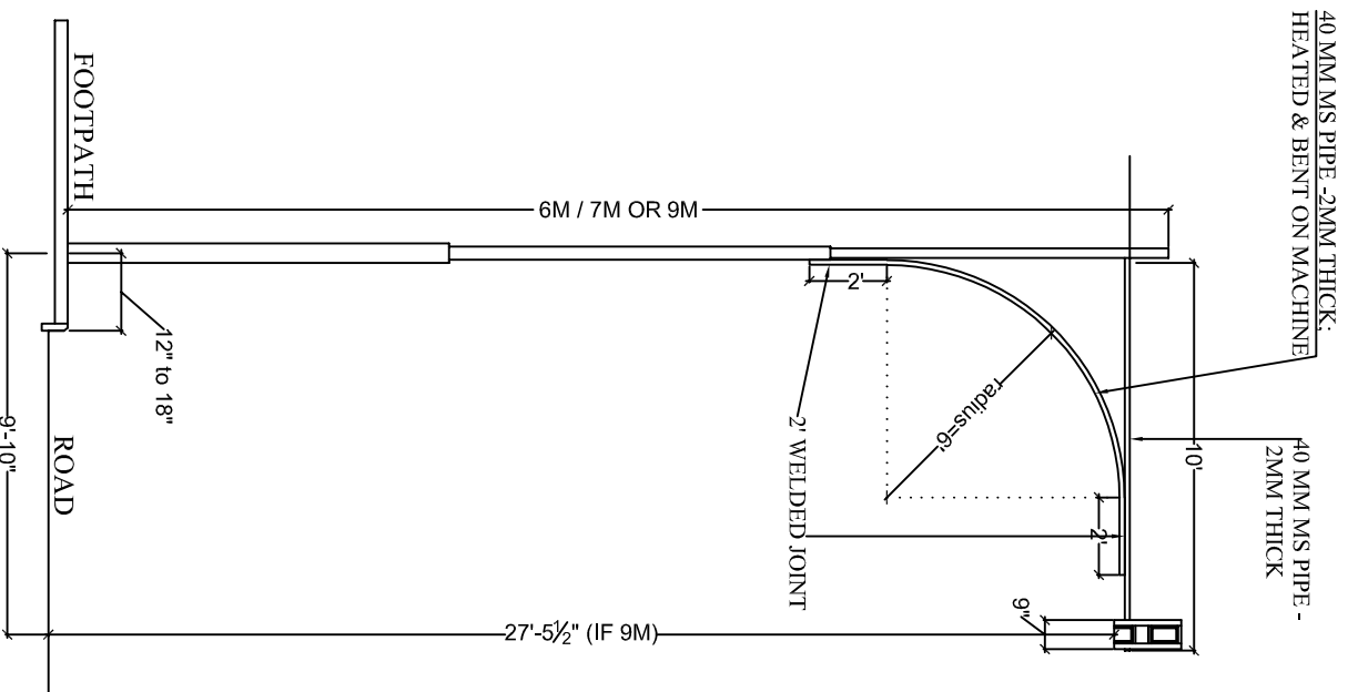
SIDE VIEW
