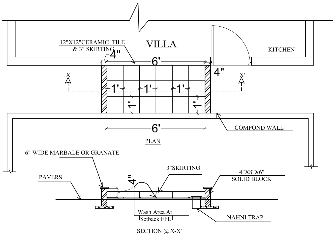
DETAIL @ A
