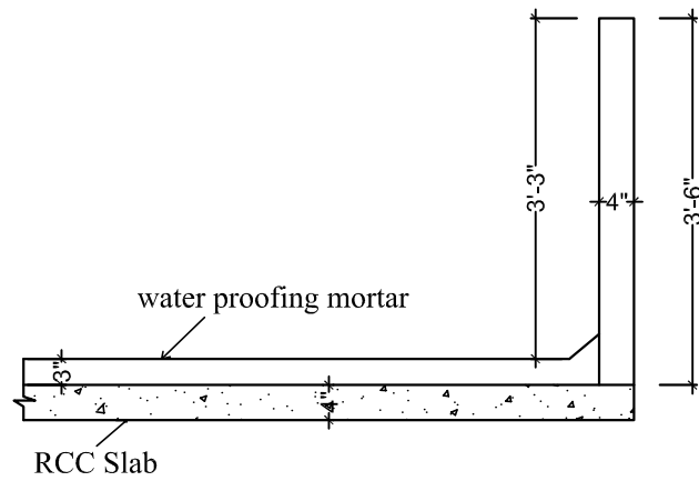
PARAPET WALL
