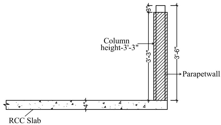
PARAPET WALL
