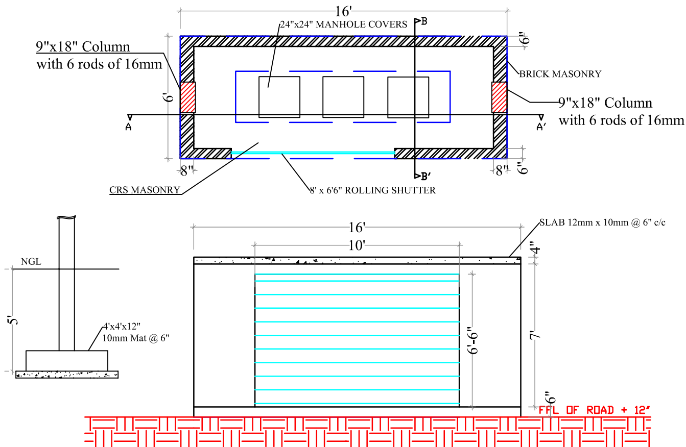
FRONT ELEVATION
