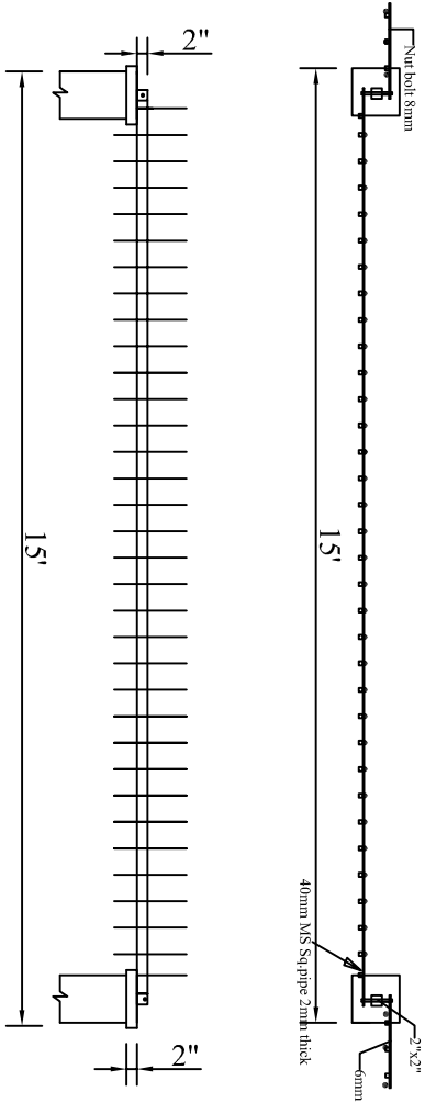
Compound wall fencing-Type I
