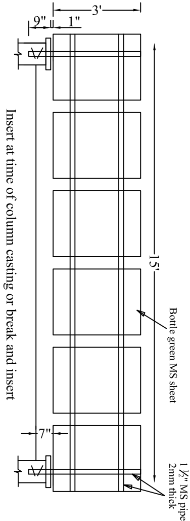
Compound wall fencing-Type II
