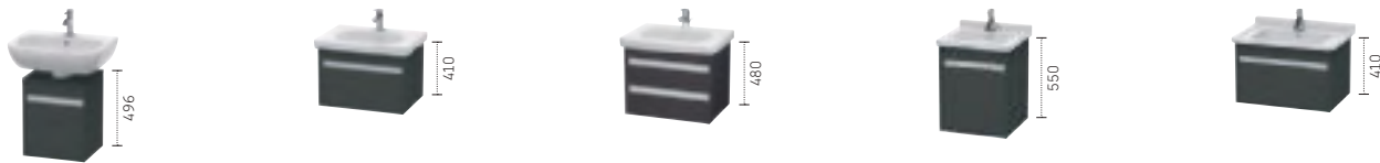
Vanity units D-Code ↔ 400 ↗ 360 # KT 6658 L/R Plinth legs # KT 9911 D-Code ↔ 600 ↗ 455 # KT 6670 ↔ 800 ↗ 455 # KT 6667 ↔ 1000 ↗ 455 # KT 6668 D-Code ↔ 600 ↗ 455 # KT 6650 ↔ 800 ↗ 455 # KT 6647 ↔ 1000 ↗ 455 # KT 6648 Starck 3 ↔ 440 ↗ 455 # KT 6662 L/R Starck 3 ↔ 650 ↗ 465 # KT 6663 ↔ 800 ↗ 465 # KT 6664 ↔ 1000 ↗ 465 # KT 6665
