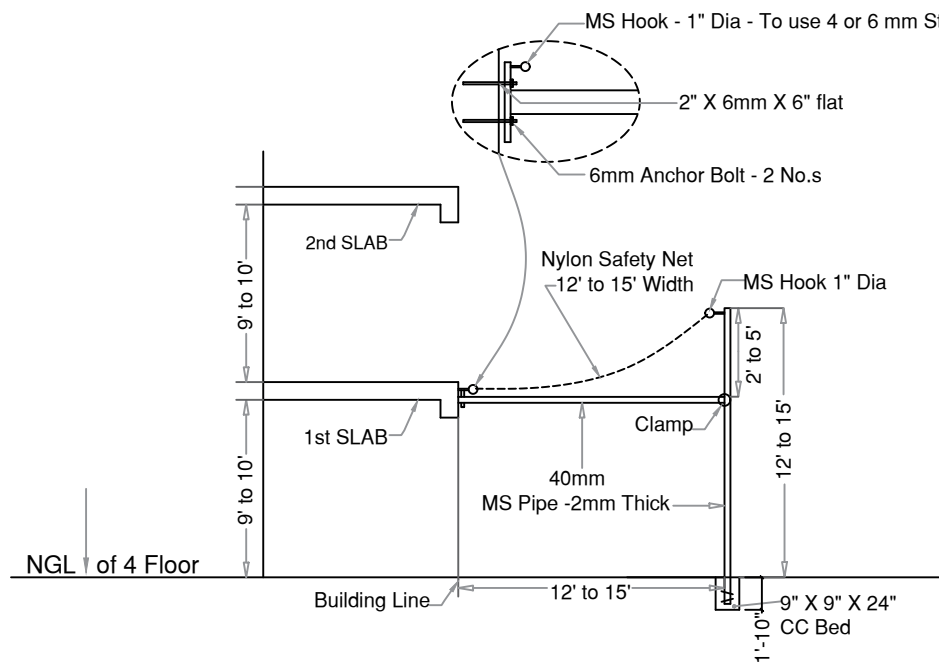
ELEVATION [OPTION - 1]
