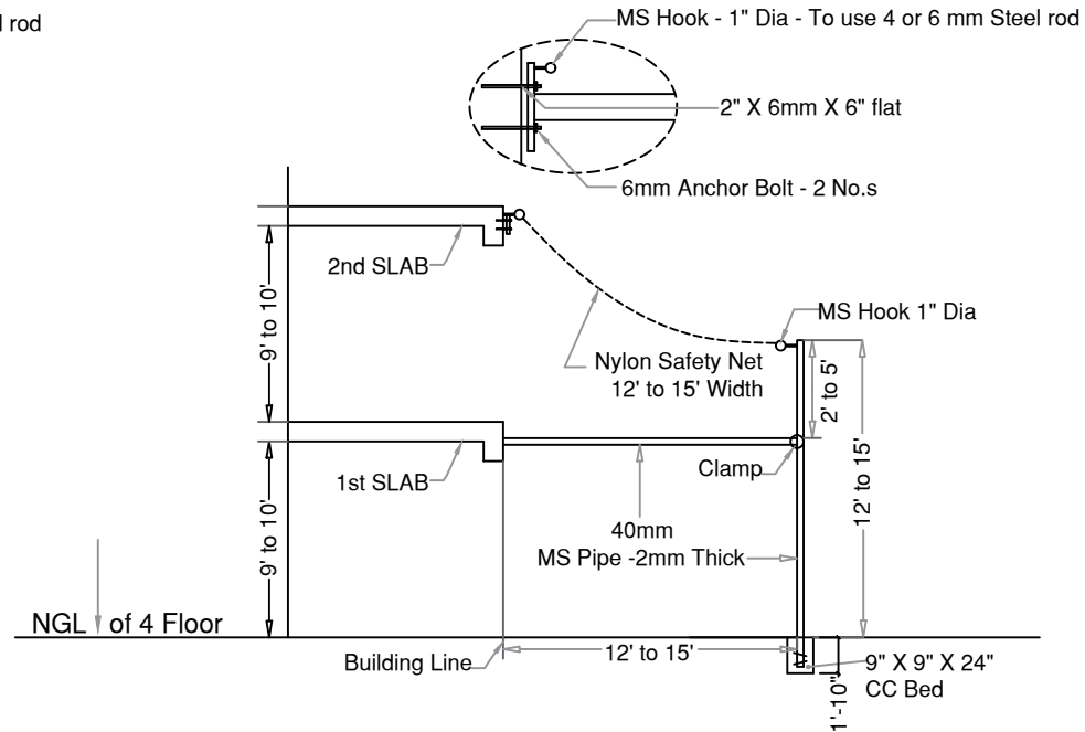
ELEVATION [OPTION - 2]
