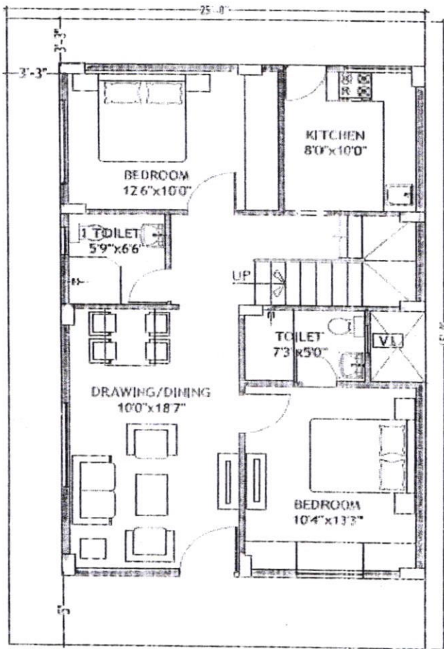
GROUND FLOOR PLAN AREA: 800 SFT
