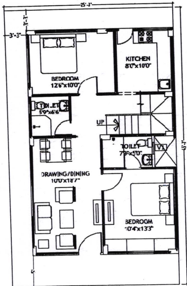
GROUND FLOOR PLAN AREA: 800 SFT
