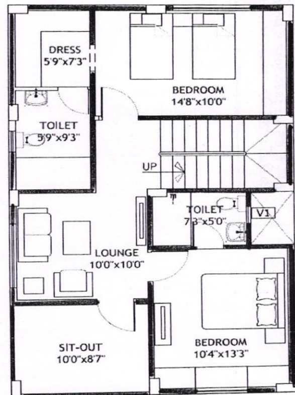
FIRST FLOOR PLAN AREA: 800 SFT
