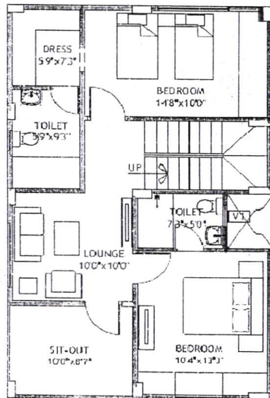
FIRST FLOOR PLAN AREA: 800 SFT
