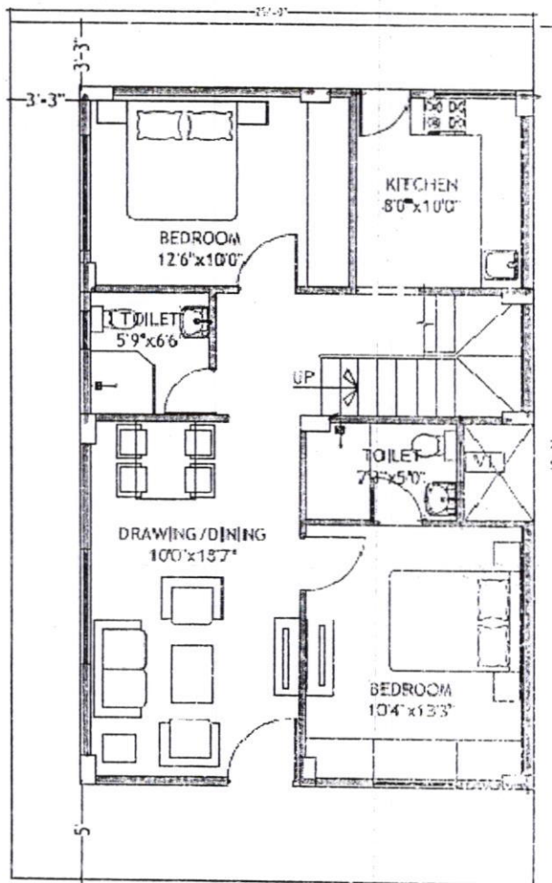
GROUND FLOOR PLAN AREA: 800 SFT
