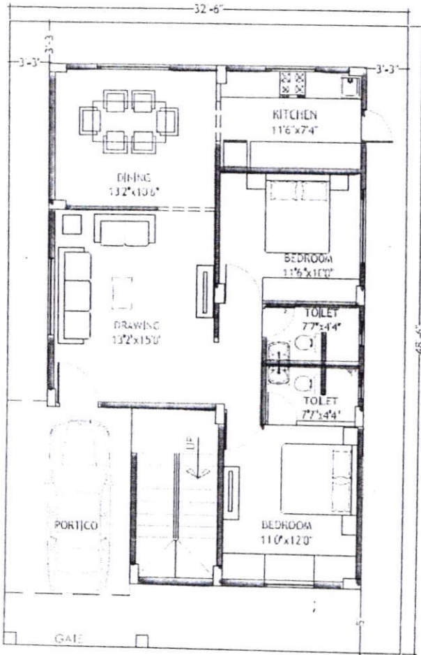
GROUND FLOOR PLAN AREA: 1100.00 SFT
