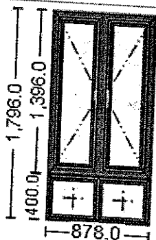
View from inside. Opens outwards.
