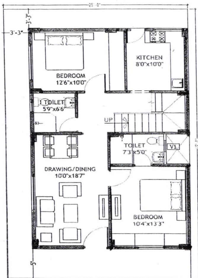
GROUND FLOOR PLAN AREA: 800 SFT
