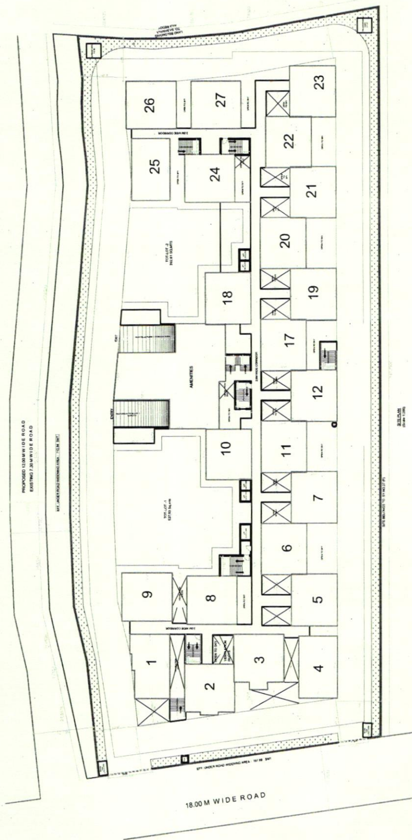
Layout plan of the Housing Project:
