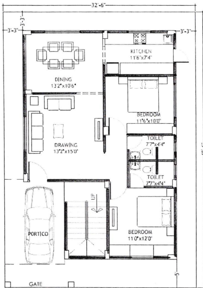
GROUND FLOOR PLAN AREA: 1100.00 SFT
