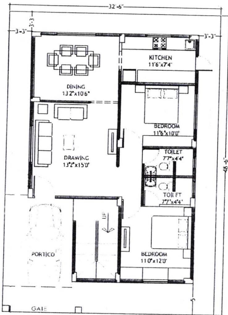
GROUND FLOOR PLAN AREA: 1100.00 SFT
