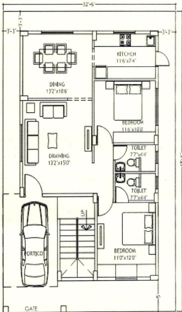
GROUND FLOOR PLAN AREA: 1100.00 SFT
