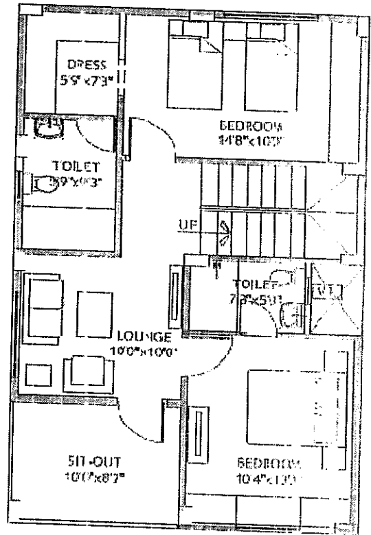
FIRST FLOOR PLAN AREA: 800 SFT
