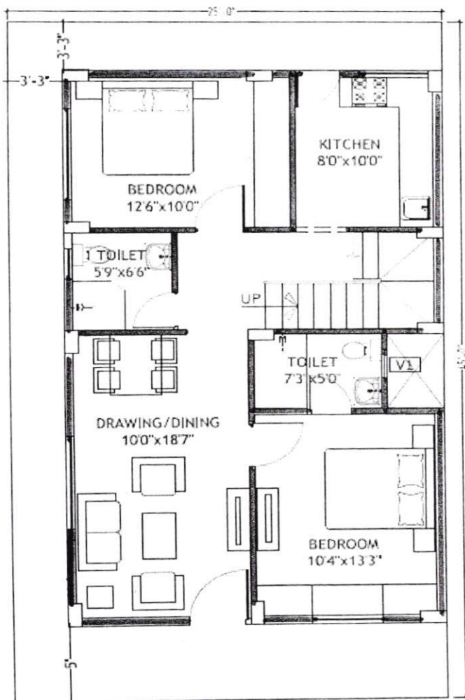
GROUND FLOOR PLAN AREA: 800 SFT
