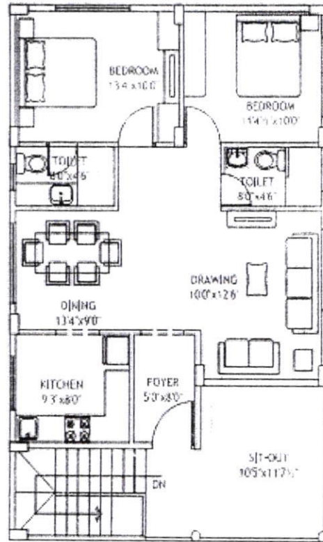
FIRST FLOOR PLAN AREA: 1050 SFT
