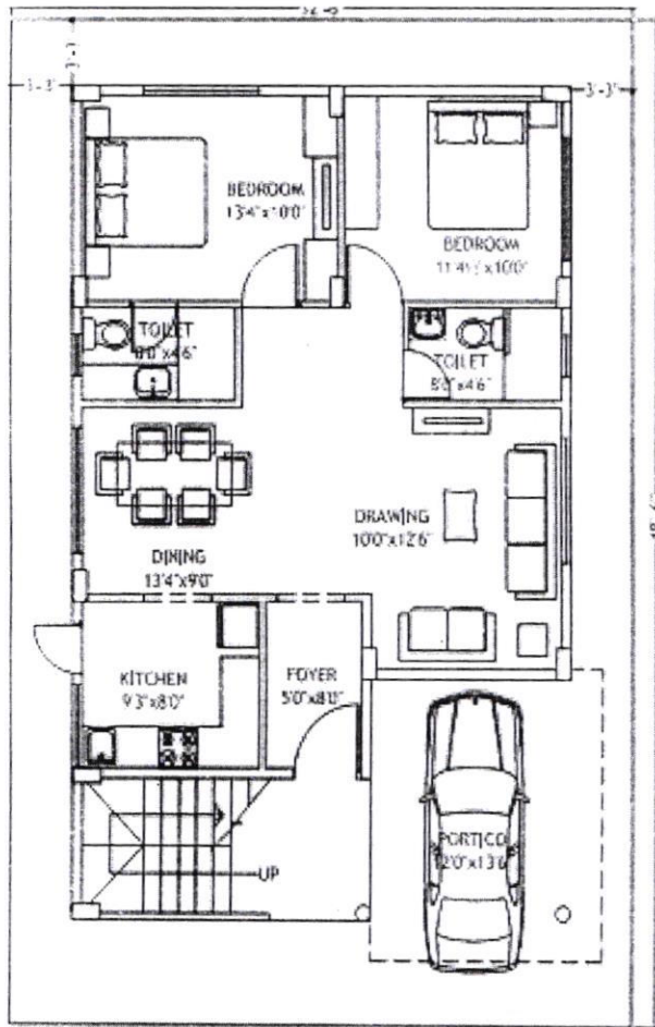
GROUND FLOOR PLAN AREA: 1100 SFT
