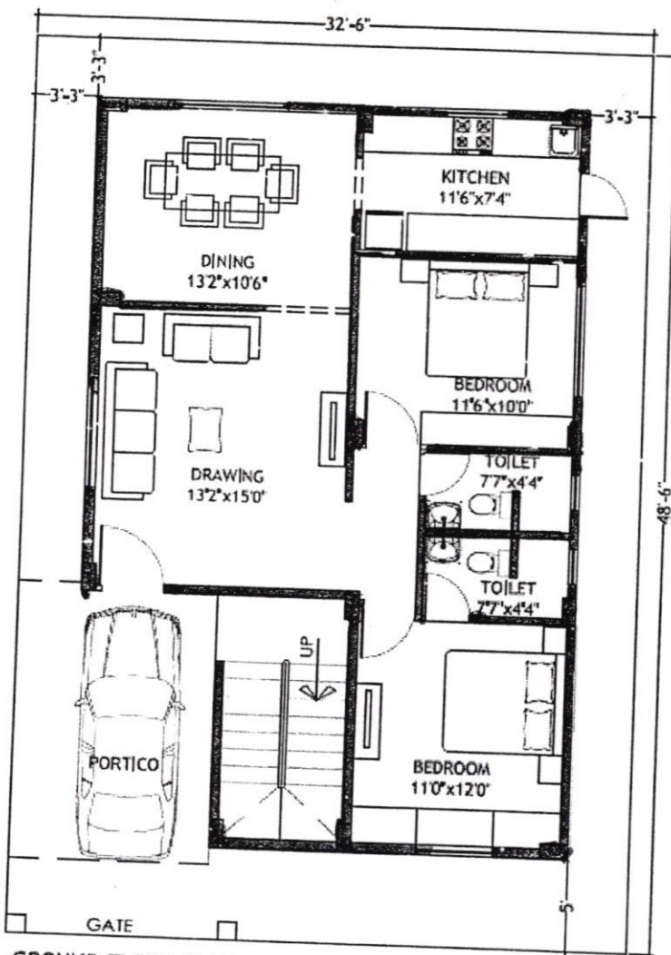
GROUND FLOOR PLAN AREA: 1100.00 SFT
