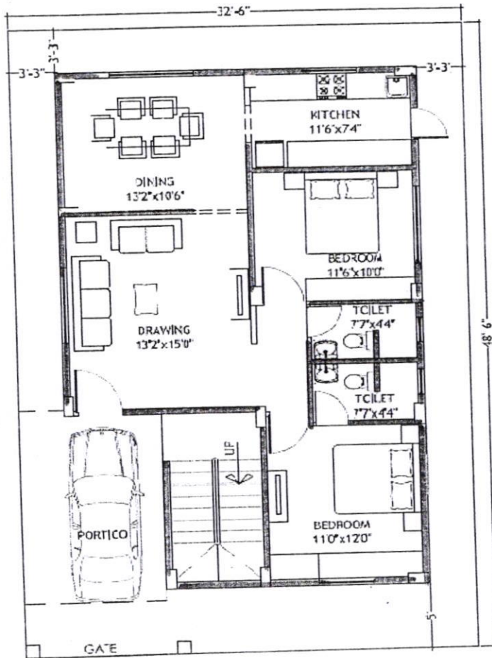
GROUND FLOOR PLAN AREA: 1100.00 SFT
