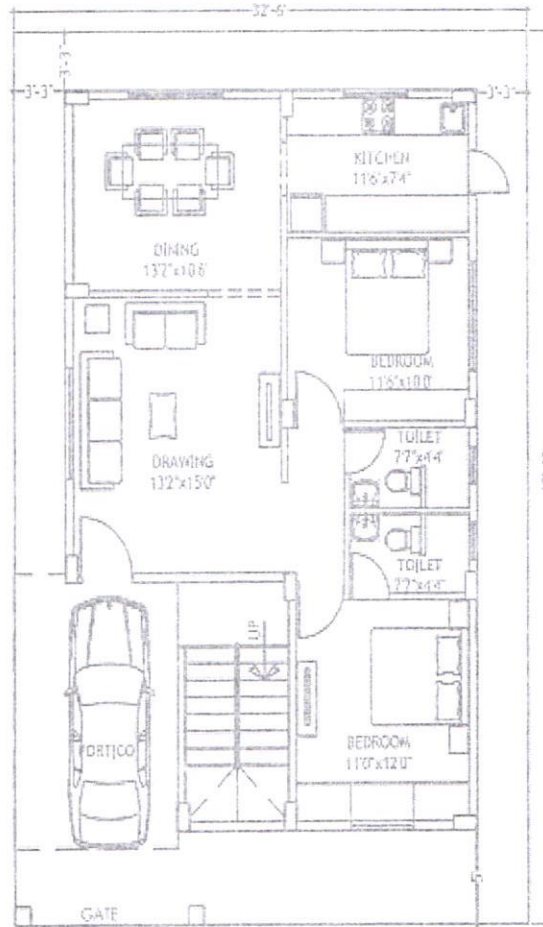
GROUND FLOOR PLAN AREA: 1100.00 SFT
