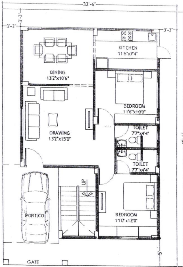
GROUND FLOOR PLAN AREA: 1100.00 SFT
