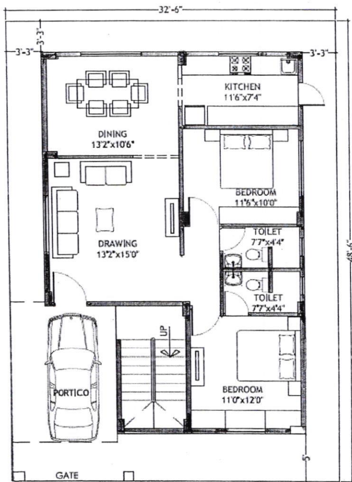
GROUND FLOOR PLAN AREA: 1100.00 SFT
