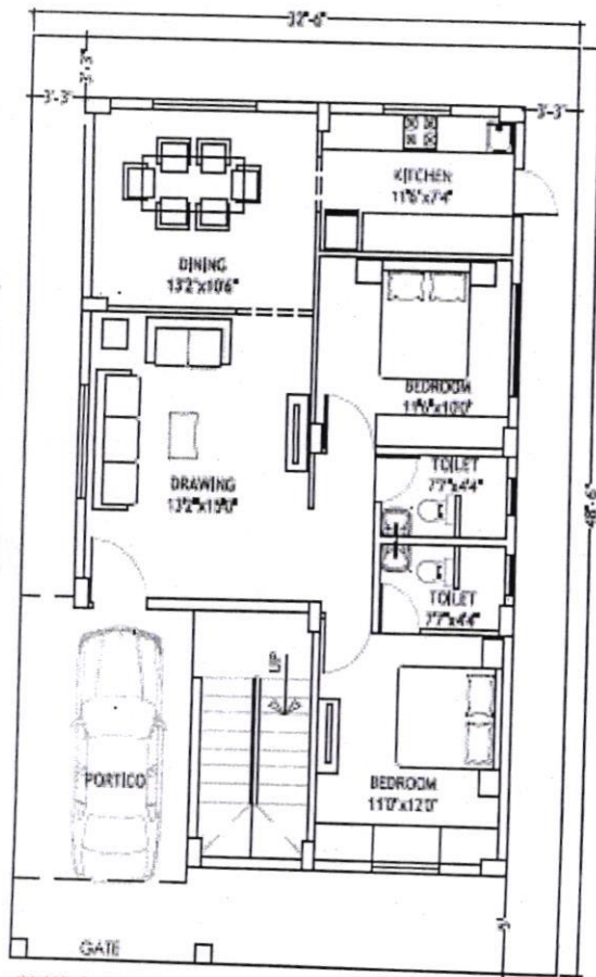
GROUND FLOOR PLAN AREA: 1100.00 SFT
