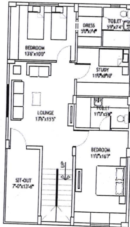
FIRST FLOOR PLAN AREA: 1050.00 SFT
