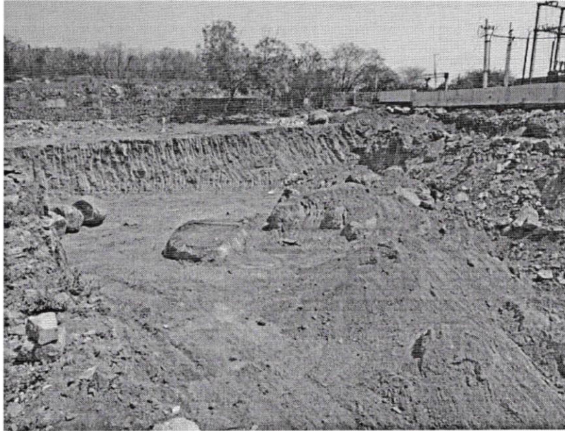
Photograph -7: Rock Stratum in the form of Huge boulders near to borehole BH-3
