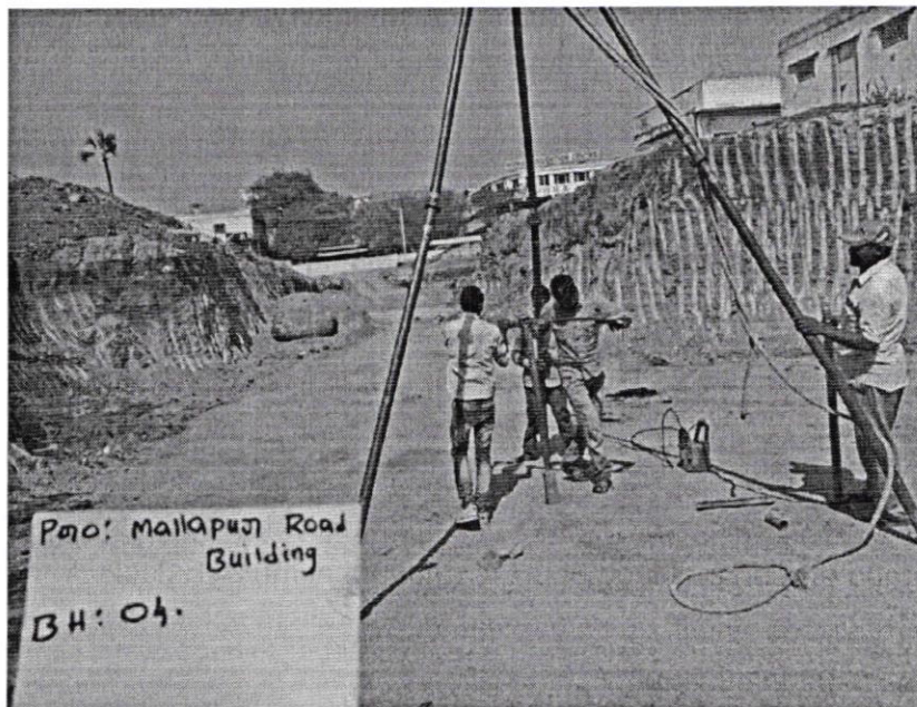
Photograph -8: Auger Borehole under progress at borehole BH-4
